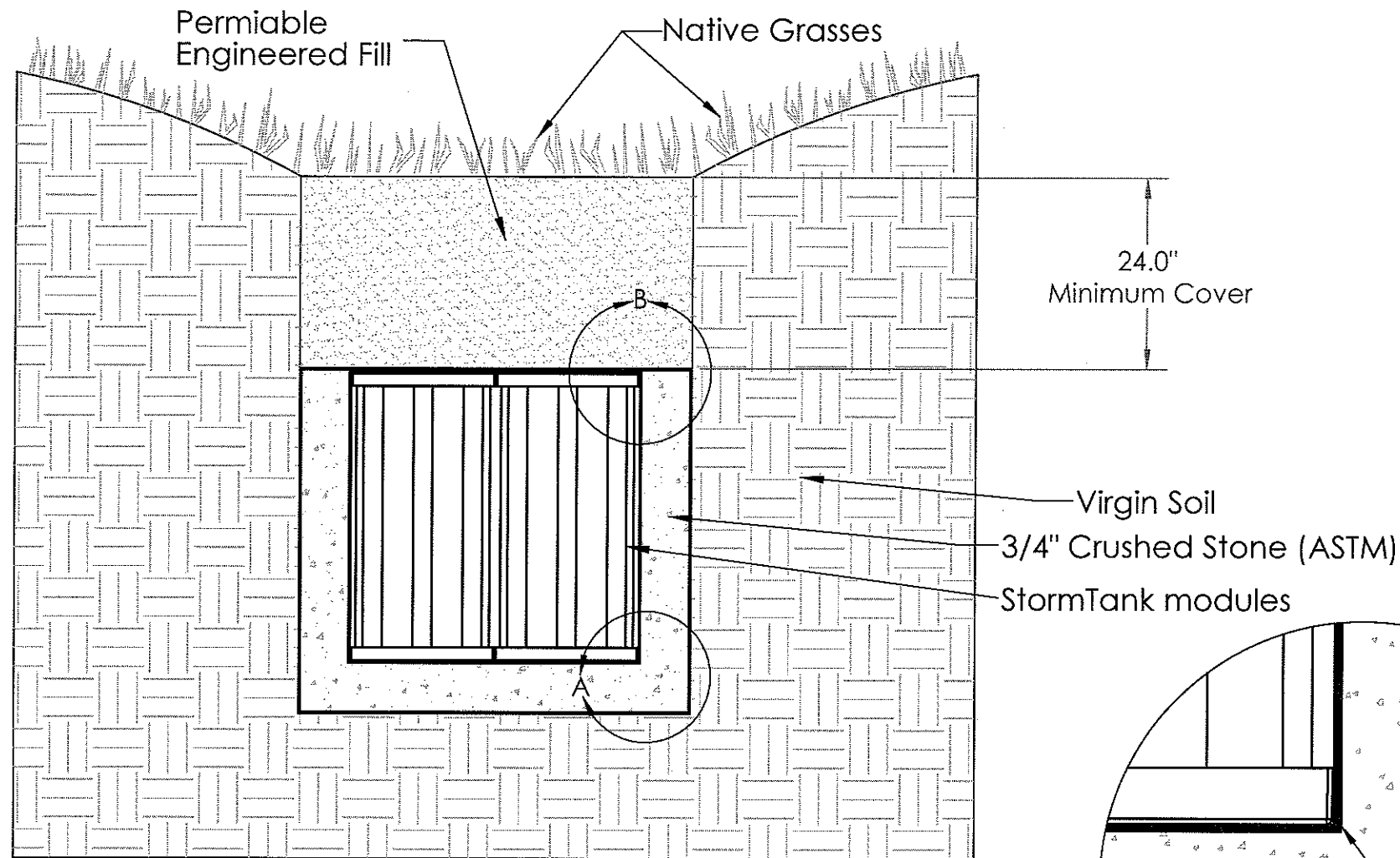
Front View
